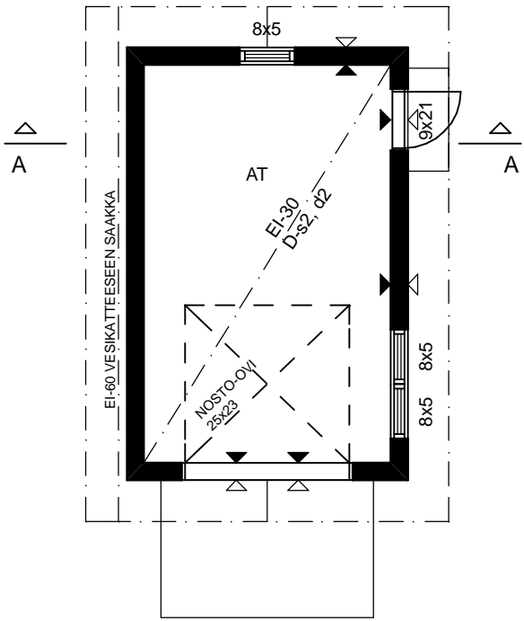
AT KERROSALA (US250mm) 26m 2 TILAVUUS 80m 3
